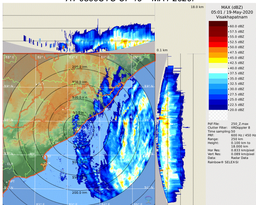
FIGURE(BELOW): REFLECTIVITY OF VISHAKHAPATNAM DOPPLER WEATHER RADAR AT 0500UTC OF 19 TH MAY 2020.
