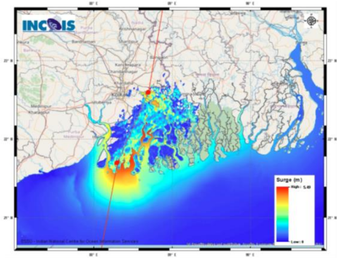
FIGURE: STORM SURGE FORECAST FROM INCOIS ISSUED AT 0600 UTC OF 19 TH MAY 2020
